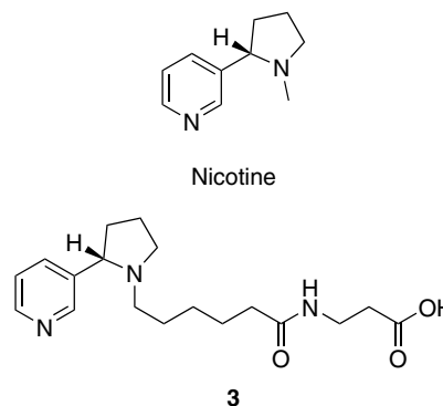
Figure 1. Structures of nicotine and structurally congruent hapten 3 used to elicit tight binding nicotine antibodies.
