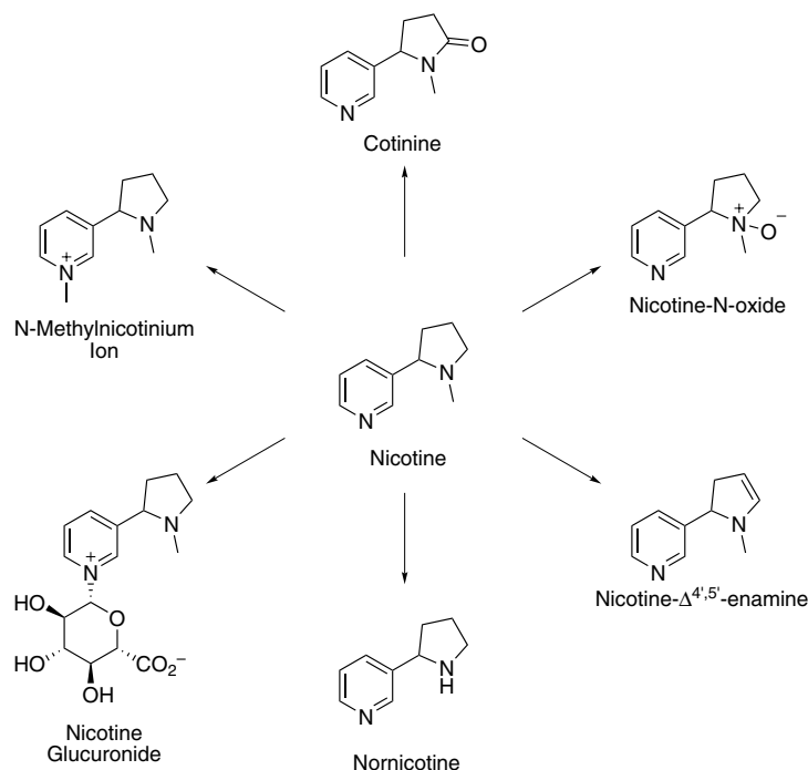
Scheme 1. The six major metabolites of nicotine in mammals. The major metabolites, cotinine, and nicotine- N -oxide, are clearly derived from oxidation processes, but all are synthesized via formal oxidations.
