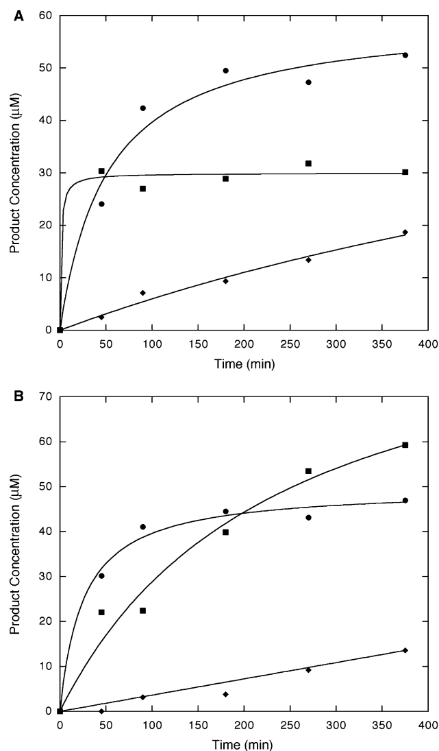
Figure 2. Time course plots of the formation of 1 (A) and 2 (B). Filled circles: TD1-10E8, riboflavin, nicotine, and visible light; Filled squares: TD1-36H10, riboflavin, nicotine, and visible light; Filled diamonds: riboflavin, nicotine, and visible light. Data was fit using Kaleidagraph 3.0.5 (Abelbeck software) using nonlinear regression analysis.
