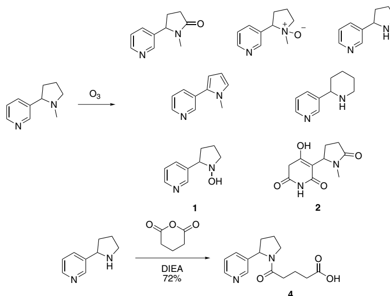
Scheme 2. Chemical ozonation of nicotine and hapten 4 used to elicit nicotine-binding antibodies.
